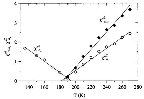
FIG. 6. \chi''_{\min}^2 vs T ( \blacklozenge , T > T_C ) and \chi''_{\sigma}^2 vs T ( \circ , T \geq T_C ). Extrapolation to \chi''=0 gives T_C=187 \pm 5 K.
