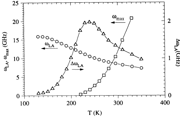
FIG. 17. Temperature dependence of the LA mode peak frequency \omega_{\text{LA}} (○) and linewidth \Delta\omega_{\text{LA}} (△), and the \alpha -relaxation peak frequency \omega_{\text{max}} (□) in the depolarized spectra of Fig. 7. The maximum width of the LA mode occurs at T \sim 240 K. At this temperature, the \alpha -peak frequency \omega_{\text{max}} is about five times smaller than the LA mode peak frequency.
